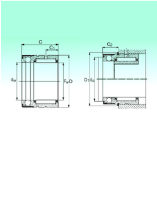
NX 12 Z Bearing 2D drawings and 3D CAD models
